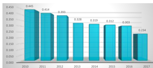
Treated Wastewater Disposal / Quantity of produced products ( m^3 / MT)
