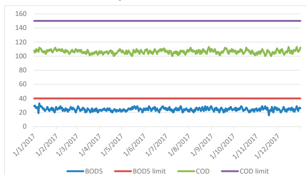
BOD 5 / COD Measurements
