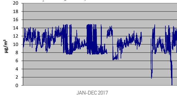
H 2 S Average hourly values - Mobile Station
