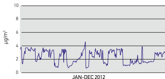
H 2 S AVERAGE DAILY VALUES - STATION T752
