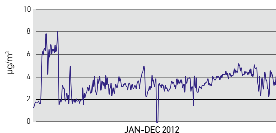
H 2 S AVERAGE DAILY VALUES - MOBILE STATION
