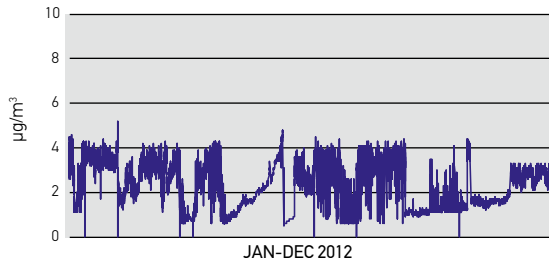
H 2 S AVERAGE HOURLY VALUES - STATION AVIN
