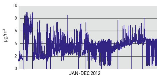
H 2 S AVERAGE HOURLY VALUES - MOBILE STATION
